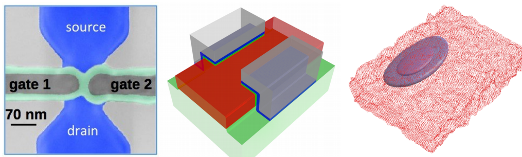
(Left) A SOI device with two “face to face” gates, each one controlling a quantum dot beneath. The information is encoded as a superposition of the up and down spin states of the carrier(s) trapped in these dots. (Middle) The same device as modeled in TB_Sim, with silicon in red, \text{SiO}_2 in green, \text{HfO}_2 in blue and the gates in gray. (Right) Iso-probability surfaces of the ground-state wave function under the leftmost gate; each red dot is a silicon atom at the surface of the channel (surface roughness is included in this simulation).
